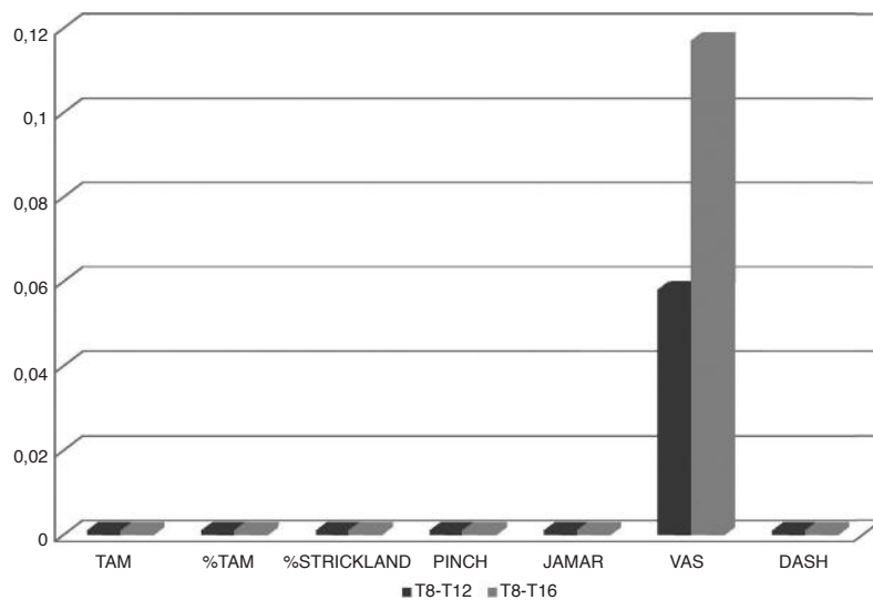
Grafico 7. Paired student t-test.
